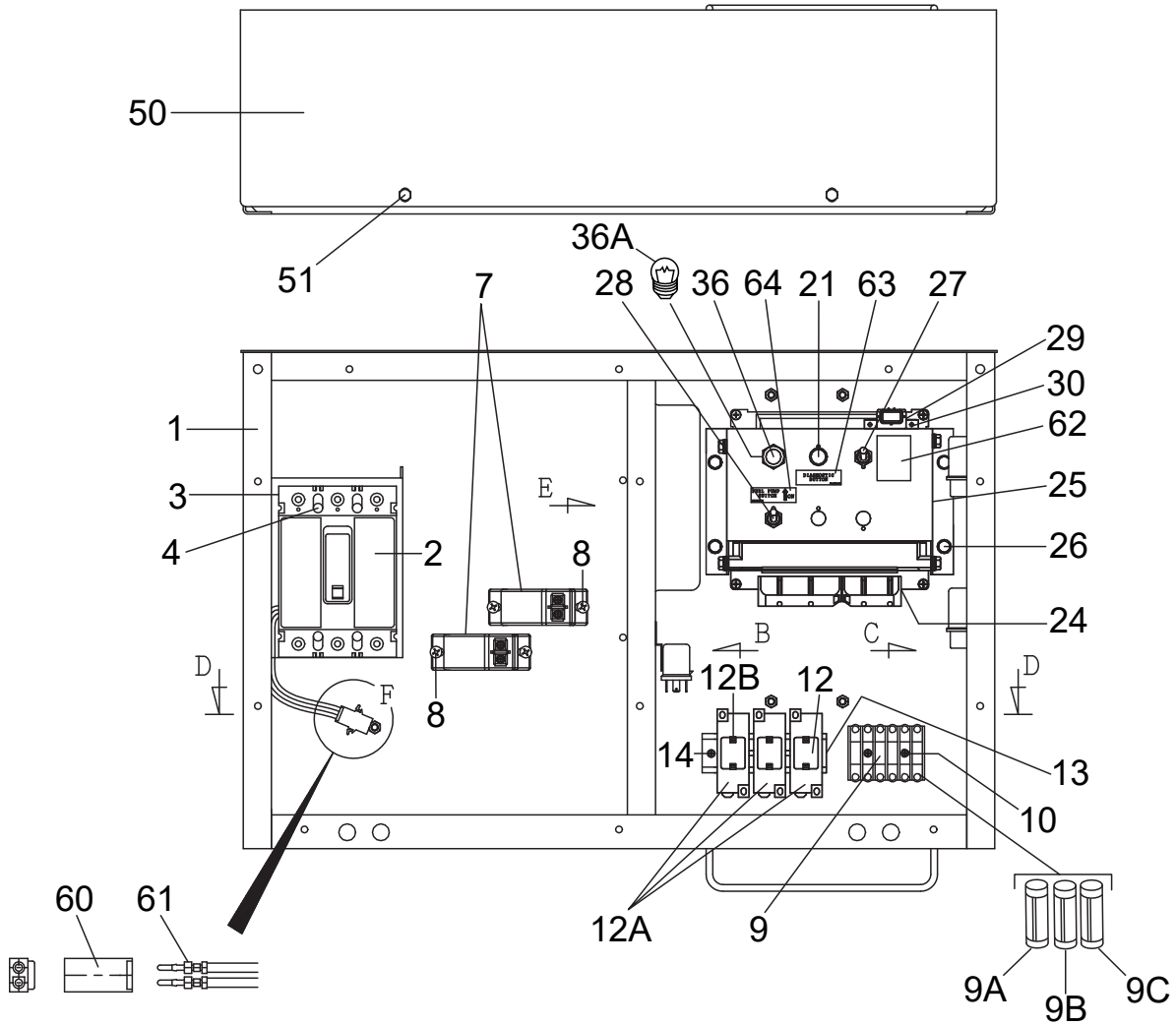
DETAIL-F
